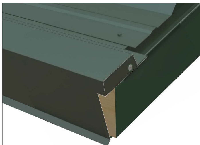
Figure 49. Ends Folded and Riveted
