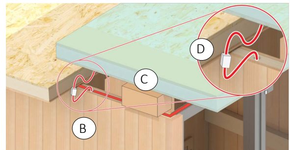
Figure 18. Placing the Front Roof and Cable Connection
