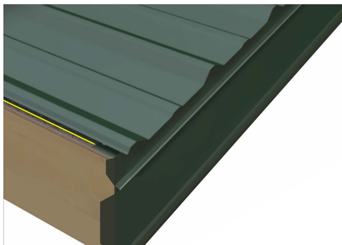
Figure 43. Aligning Edge with Chalk Line
