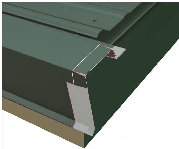
Figure 48. Cuts, Waste Pieces, and Folds Marked
