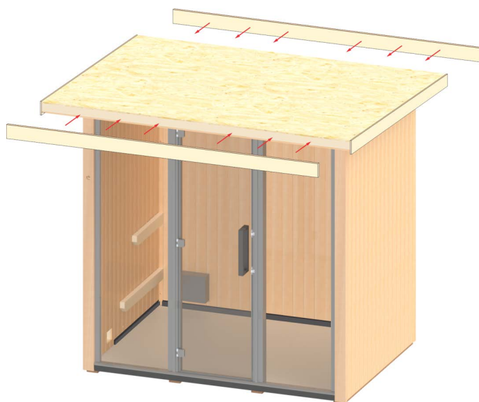
Figure 22. Installing Front and Back Wood Fascia
