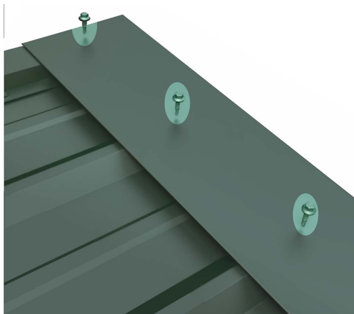
Figure 53. Attaching Front Edge Cap
