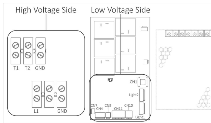
Figure 54. CB Box Interior
