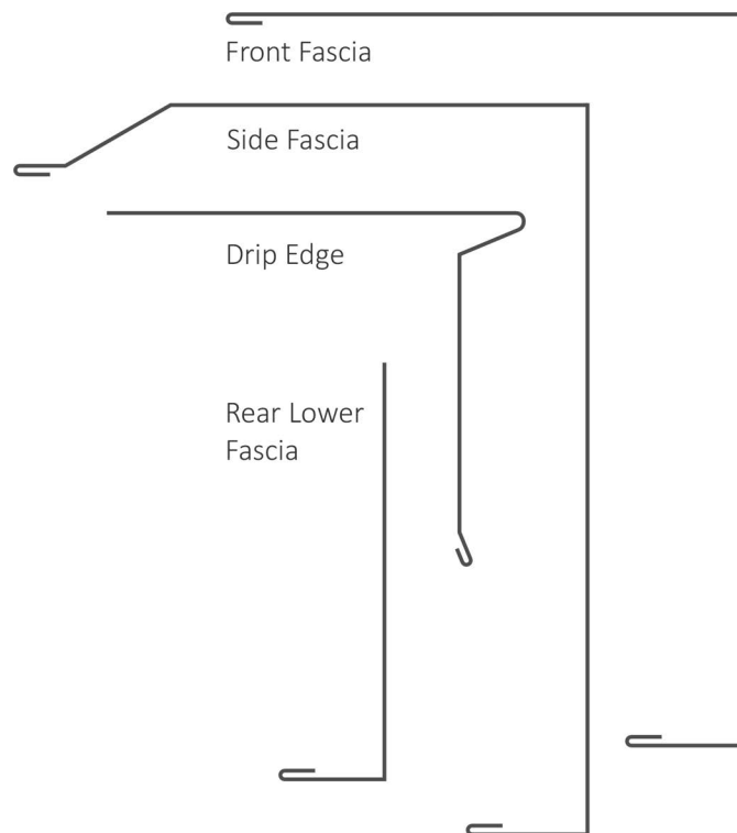
Figure 37. Metal Fascia Profiles
