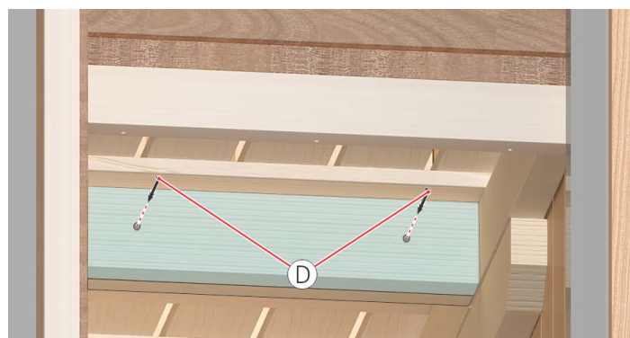
Figure 30. Attaching the Return Bench
