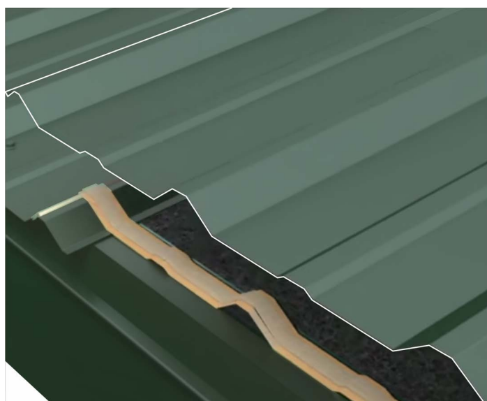
Figure 45. Aligning and Laying Second Sheet
