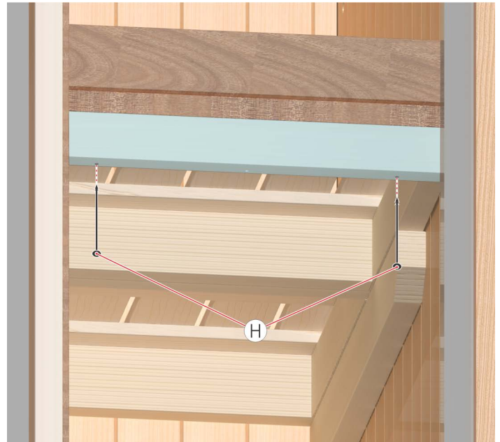
Figure 33. Attaching Armrest to Return Bench
