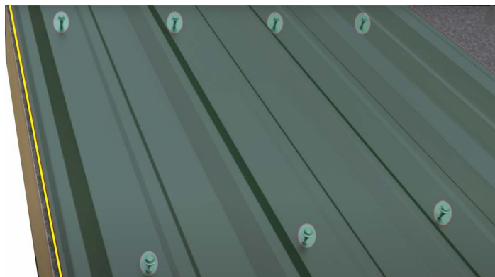
Figure 44. Attaching the Metal Roofing
