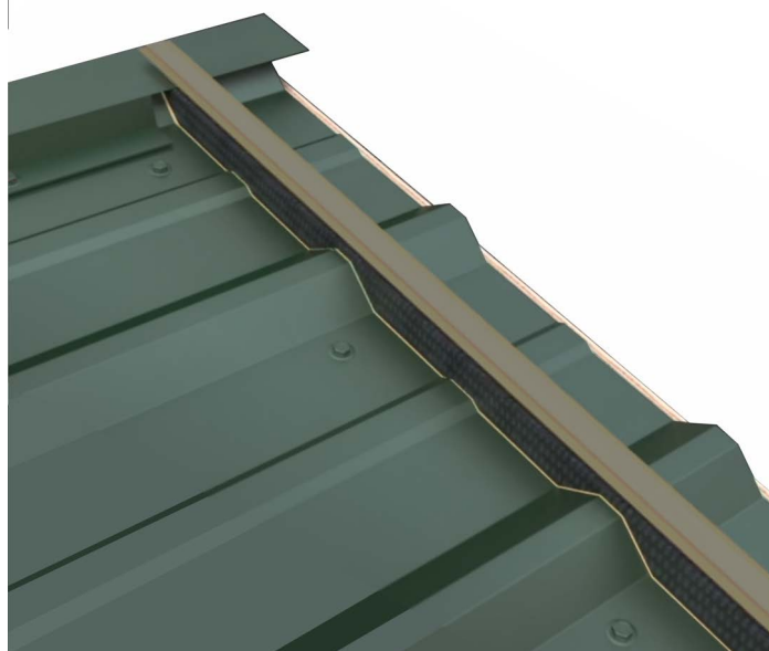
Figure 51. Applying Polyethylene Closure and Tape
