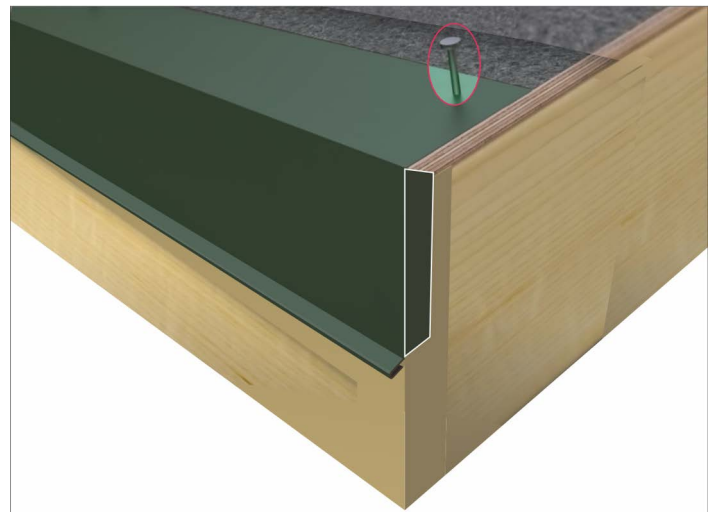
Figure 39. Applying Drip Edge
