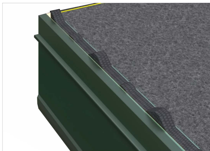
Figure 42. Applying Polyethylene Closure
