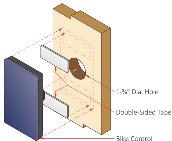
Figure 55. Mounting the Control
