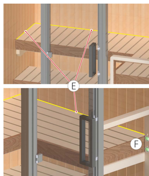
Figure 31. Equalizing Bench-to-Wall Spacing
