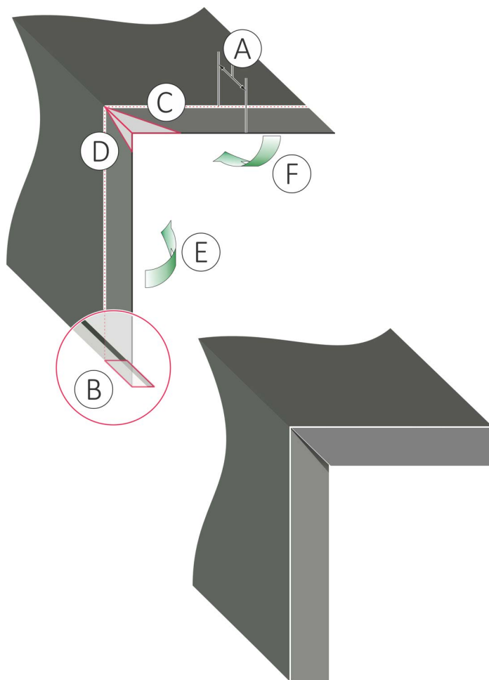
Figure 52. Folding Ends of Front Edge Cap
