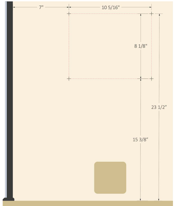
Figure 35. Heater Mounting Measurements
